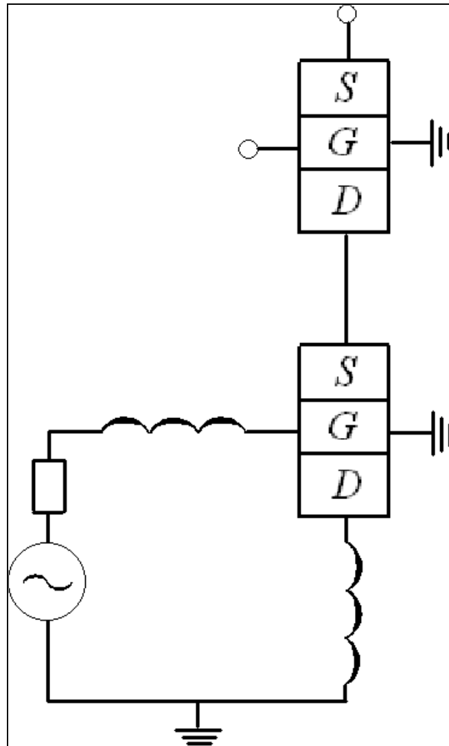
Fig 1a: Structure of the cascode amplifier [24]
