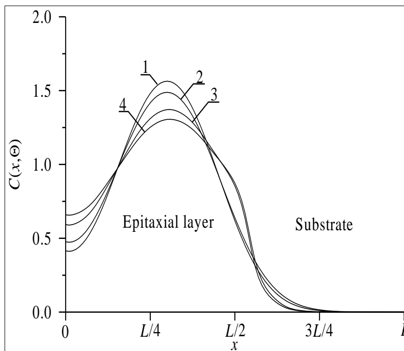
Fig3: Distributions of concentration of implanted dopant in heterostructure from Fig. 1 in direction, which is perpendicular to interface between epitaxial layer substrate. Curves 1 and 3 corresponds to annealing time \Theta = 0.0048(L_x^2+L_y^2+L_z^2)/D_0 . Curves 2 and 4 corresponds to annealing time \Theta = 0.0057(L_x^2+L_y^2+L_z^2)/D_0 . Curves 1 and 2 corresponds to homogenous sample. Curves 3 and 4 corresponds to heterostructure under condition, when value of dopant diffusion coefficient in epitaxial layer is larger, than value of dopant diffusion coefficient in substrate
