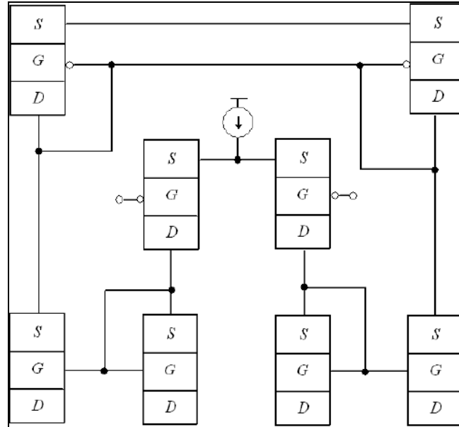
Fig 1: Structure of the considered amplifier [4] .
