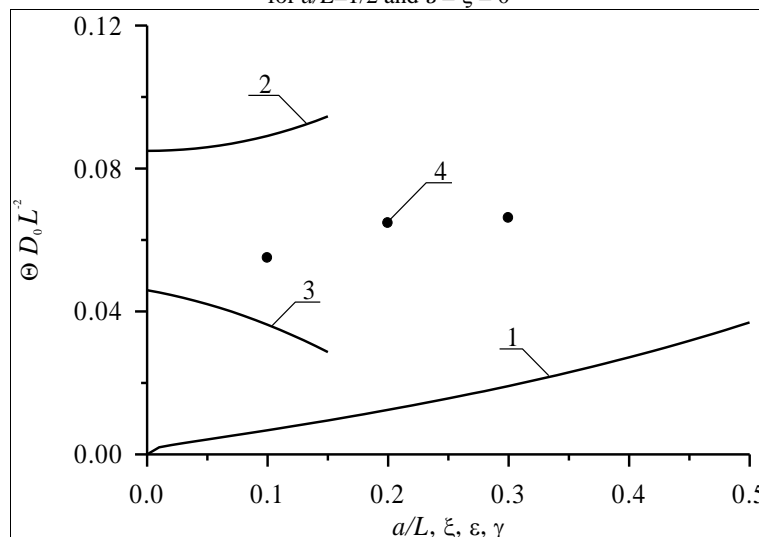
Fig 4: Dependences of dimensionless optimal annealing time for doping by ion implantation, which have been obtained by minimization of mean-squared error, on several parameters. Curve 1 is the dependence of dimensionless optimal annealing time on the relation a/L and \xi = \gamma = 0 for equal to each other values of dopant diffusion coefficient in all parts of heterostructure. Curve 2 is the dependence of dimensionless optimal annealing time on value of parameter \varepsilon for a/L=1/2 and \xi = \gamma = 0 . Curve 3 is the dependence of dimensionless optimal annealing time on value of parameter \xi for a/L=1/2 and \varepsilon = \gamma = 0 . Curve 4 is the dependence of dimensionless optimal annealing time on value of parameter \gamma for a/L=1/2 and \varepsilon = \xi = 0
