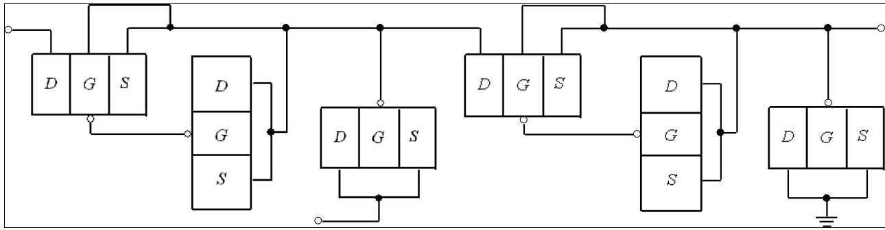
Fig 1: Structure of voltage doubler [11]. View from top
