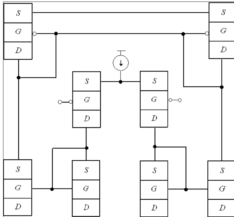
Fig 1: Structure of the considered amplifier [4]
