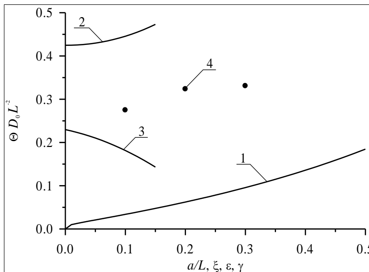
Fig 5a: Dimensionless optimal annealing time of infused dopant as a function of several parameters. Curve 1 describes the dependence of the annealing time on the relation a/L and \xi = \gamma = 0 for equal to each other values of dopant diffusion coefficient in all parts of heterostructure. Curve 2 describes the dependence of the annealing time on value of parameter \epsilon for a/L=1/2 and \xi = \gamma = 0 . Curve 3 describes the dependence of the annealing time on value of parameter \xi for a/L=1/2 and \epsilon = \gamma = 0 . Curve 4 describes the dependence of the annealing time on value of parameter \gamma for a/L=1/2 and \epsilon = \xi = 0
