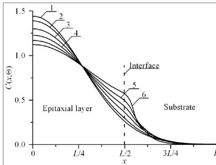
Fig 2a: Dependences of concentration of dopant, infused in heterostructure from Figs. 1, on coordinate in direction, which is perpendicular to interface between epitaxial layer substrate. Difference between values of dopant diffusion coefficient in layers of heterostructure increases with increasing of number of curves. Value of dopant diffusion coefficient in the epitaxial layer is larger, than value of dopant diffusion coefficient in the substrate
