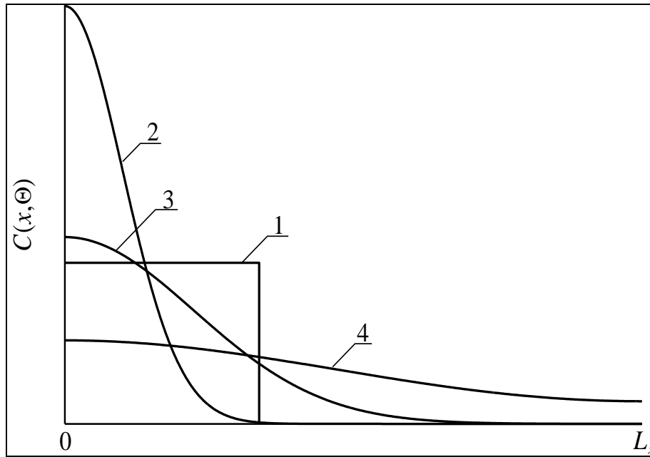
Fig. 4. Spatial distributions of dopant in heterostructure after dopant infusion. Curve 1 is idealized distribution of dopant. Curves 2-4 are real distributions of dopant for different values of annealing time. Increasing of number of curve corresponds to increasing of annealing time
